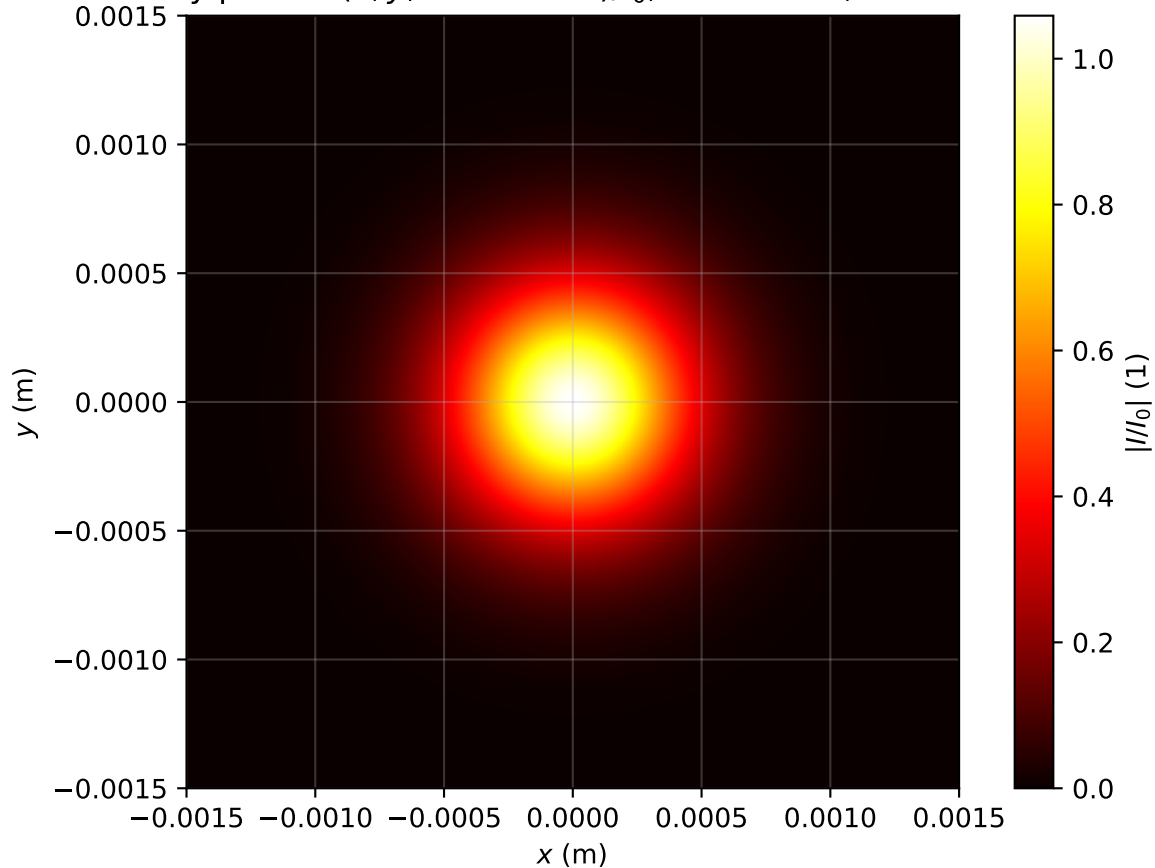
Intensity profile I(x, y, z = 0.716m)/I_0 , Pin=0.5Pcr, artificial time
